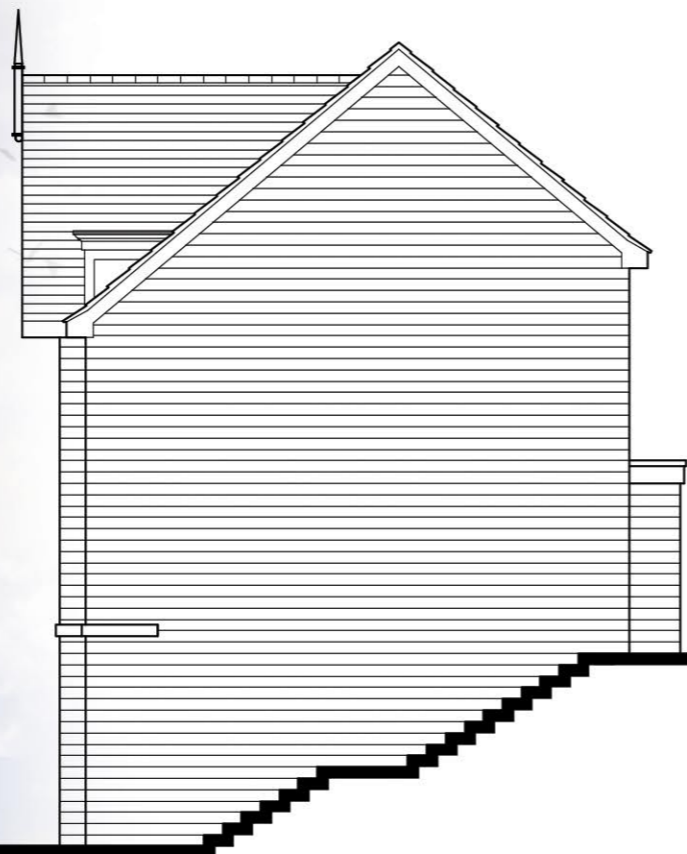
Side Elevation
